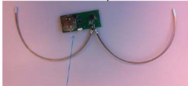
Live test shows 15dB higher RSSI with Bra-tenna versus printed IFA
